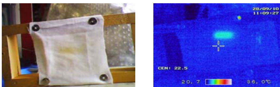
Figure 13b. Left: photo of the linen during ArF laser irradiation. On the right, the same frame seen in infrared light. The color scale reveals that the warmest area of the linen (in the middle of the laser spot) is at 25 ^\circ\text{C} , while the non-irradiated area is at the room temperature of 21 ^\circ\text{C} .
