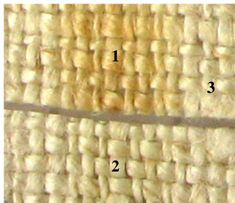
Figure 8. Linen fabric cut after irradiation below-threshold for coloration. 1) Irradiated area after heating. 2) Irradiated area not heated. 3) Not irradiated area. Latent coloration of the linen area irradiated below threshold appears only after artificial aging of the upper part of irradiated linen.
