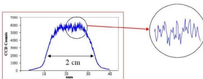
Figure 15. One-dimensional intensity/fluence profile of our laser beam measured by a CCD camera, model DV-430UV Andor, with a 22- \mu\text{m} single-pixel resolution. The inset shows an enlargement of the high-frequency spatial fluctuations.
