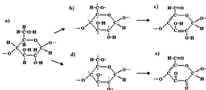
Figure 14. a) Main molecular structure common to both cellulose and hemicellulose. There are two possible transitions (a) → (b) → (c) and (a) → (d) → (e) that generate chromophores after oxidation and dehydration. The C=C and C=O double bonds in (c) and (e) act as the chromophore and are responsible for the yellow color of the fibers of image on the Shroud of Turin.
