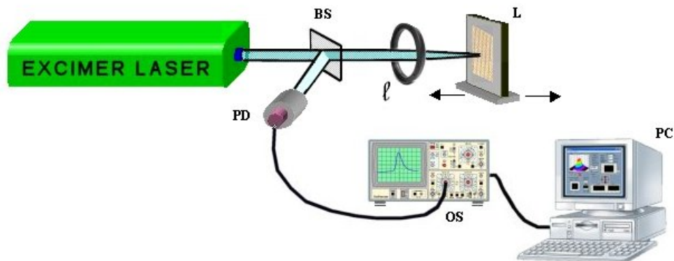
Figure 2. Setup of excimer laser irradiations of linens. The laser pulses are focused by the lens \ell on the linen fabric L . The laser fluence/intensity incident on the flax is varied by moving L along the optical axis of the lens. A small part of the laser pulse is reflected by the beam splitter BS and monitored by the photodiode PD and the oscilloscope OS connected to a personal computer PC , which records the train of pulses and processes the data taking into account the shot to shot energy fluctuations.
