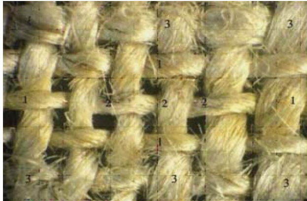
Figure 5. The area of the linen irradiated by the ArF laser beam shows different characteristics that depend on the local values of F(x,y) . 1) colored area; 2) ablated area; 3) area irradiated below the threshold for coloration.
