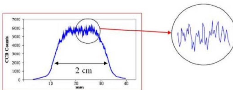
Figure 15. One-dimensional intensity/fluence profile of our laser beam measured by a CCD camera, model DV-430UV Andor, with a 22\text{-}\mu\text{m} single-pixel resolution. The inset shows an enlargement of the high-frequency spatial fluctuations.
