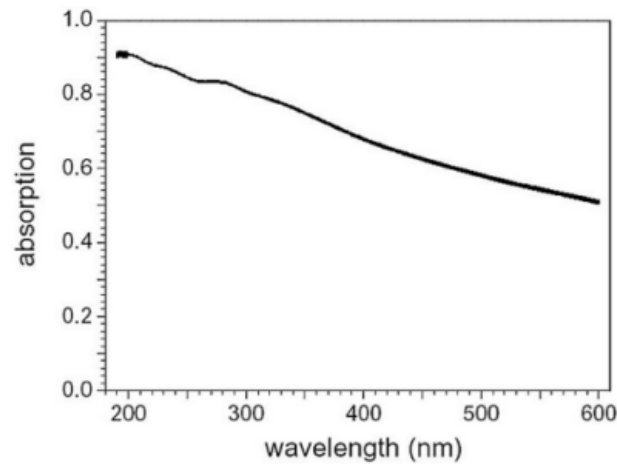
Figure 11. Plot of the absolute value of the absorbance of the linen vs. the wavelength, according with our experimental values inserted in eq. (3).
