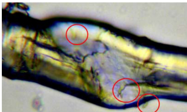
Figure 2. Microscope view of a single linen fibre mechanically damaged after it was coloured by 193-nm laser irradiation. Circles show pieces of the broken 200-nm-thin external layer of the fibril (the so called “primary cell wall”). Note these pieces are yellowish, compared with the uncoloured medulla (secondary cell wall) of the fibre. From [11].
